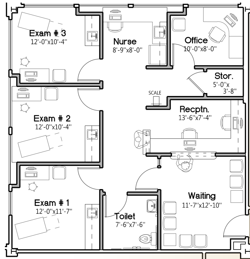
Spec Plan
